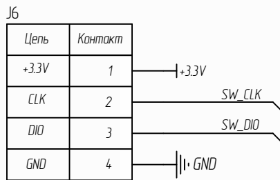
ST-LINK
